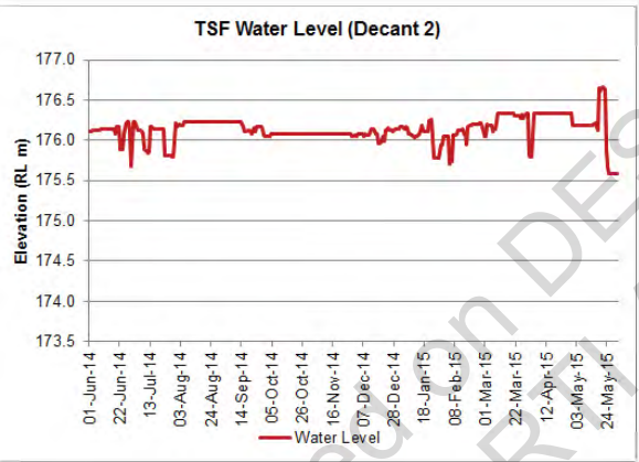
Figure 14 Tailings storage facility water level (Decant 2)
