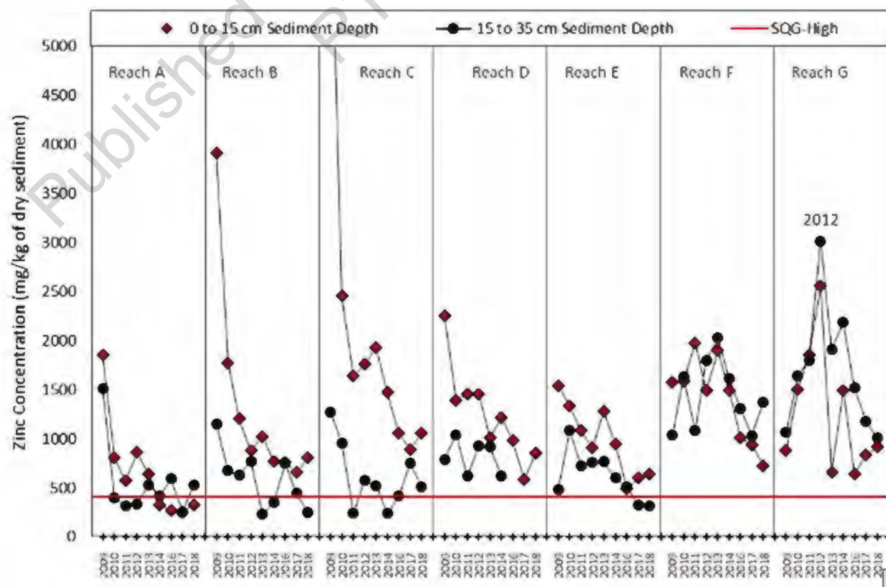
Figure 2.2.6 Variations in Page Creek zinc concentrations with sediment depth since 2009 clustered by stream reach. Points are mean values and are arranged chronologically as in Figure 2.2.5.
