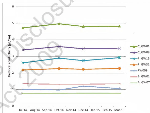
Figure 5 Groundwater electrical conductivity
