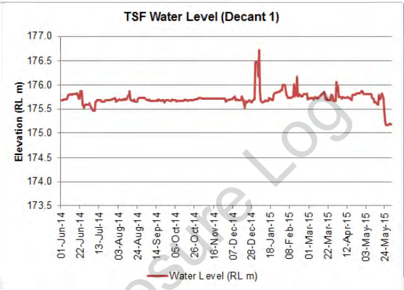
Figure 13 Tailings storage facility water level (Decant 1)
