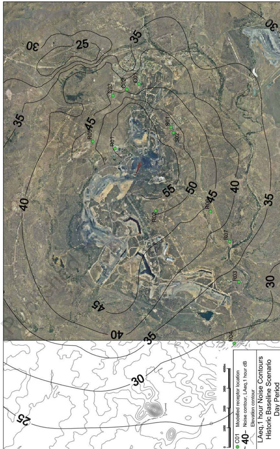
Figure 2 – Indicative 90 th Percentile Noise Contours, Historic Baseline Scenario (maximum envelope) - Day Period
