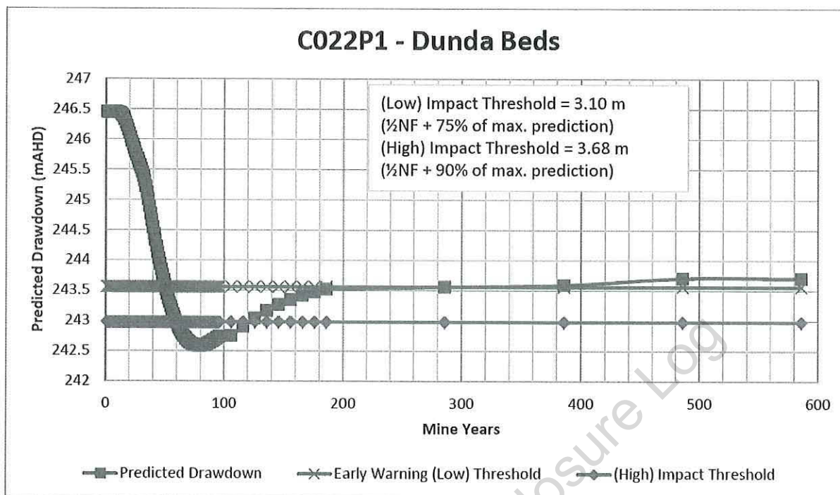
Figure 3 Plot of predicted drawdown, early warning (low) and (high) impact thresholds for bore C022P1 – Dunda Beds from Appendix E of GMMPv7
