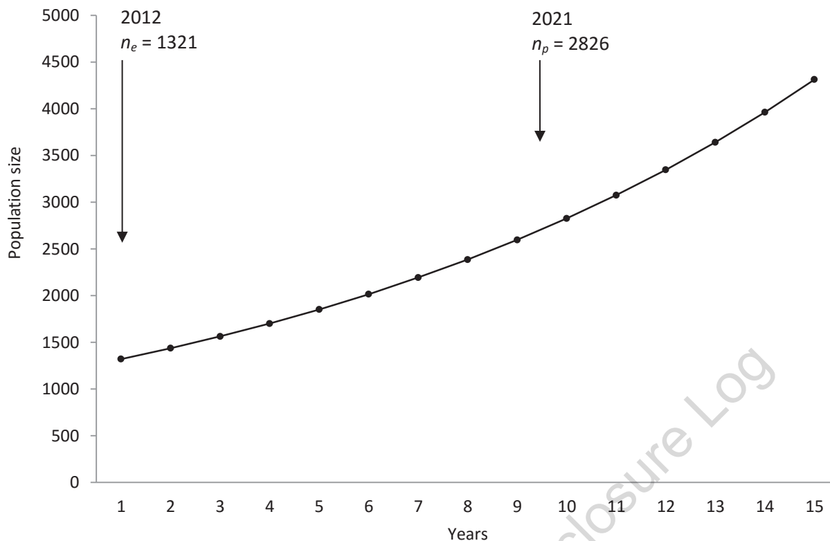
Figure 4.4: Projected population size of feral horses in the TTSTF over 15 years using the Leslie age-structured matrix simulation model. n_e – estimated population size in 2012, and n_p –projected population size in 2021.
