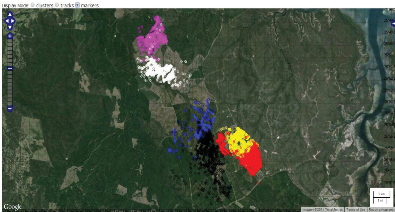
Figure 7.3: Graphical representation of home range overlap of six harems tracked by GPS in the TTSF. Large concentrations of points indicate high density data collection, which correspond to highly used plantation areas. Light green areas – open canopy habitats; dark green areas – closed canopy habitats; pink – H80; white – H88; blue – H109; black – H108; yellow – H10, and red – H12.
