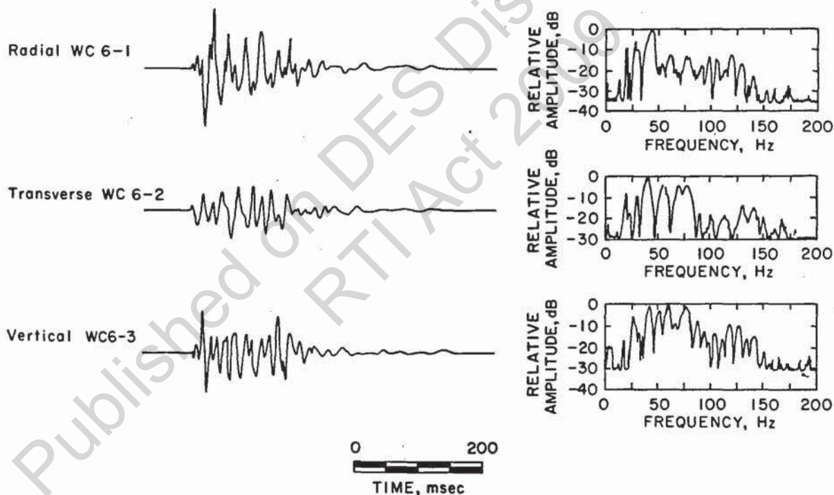
Figure 5.—Construction blast time histories and spectra measured at 75 ft.
