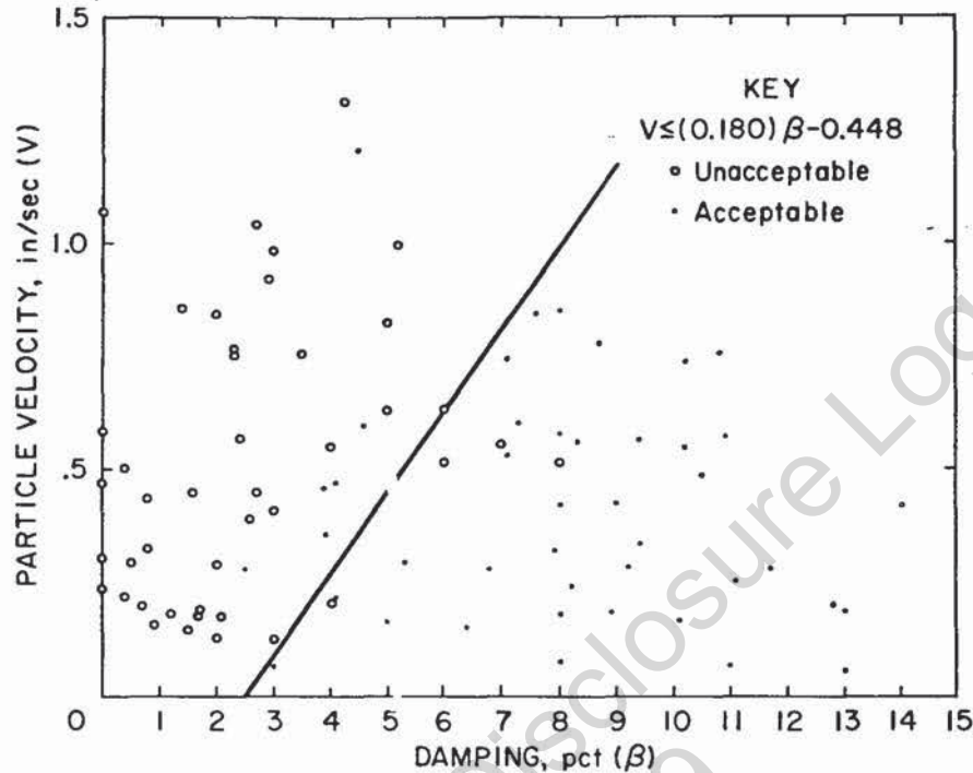
Figure 64.—Human response to vibrations of damped concrete floors, after Murray (33). Equation defines acceptable zone.
