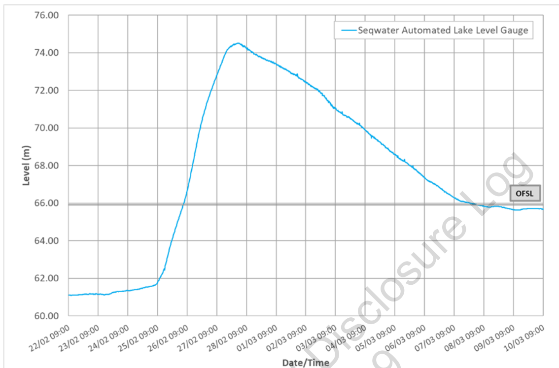
Figure 7-32: Adopted Wivenhoe Dam lake level hydrograph for reverse routing
