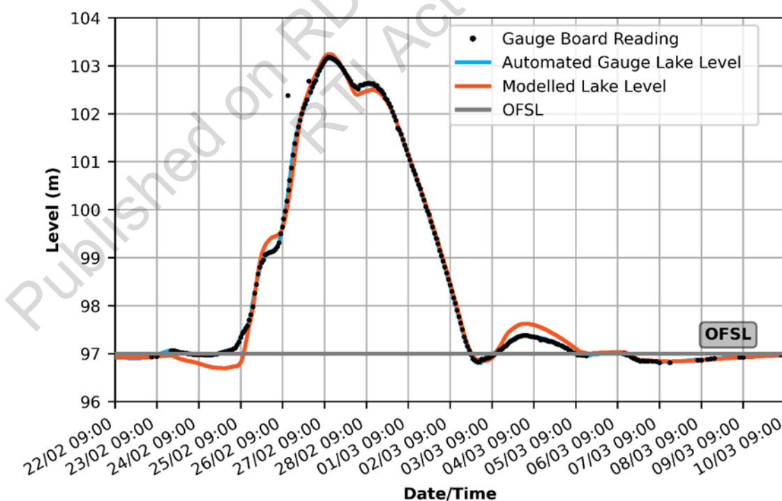
Figure 7-24: Somerset Dam post-event analysis whole of event calibration modelled lake level compared to automated data and gauge board readings for the period 22/02/2022 09:00 to 10/03/2022 09:00 (replicated in Figure v)
