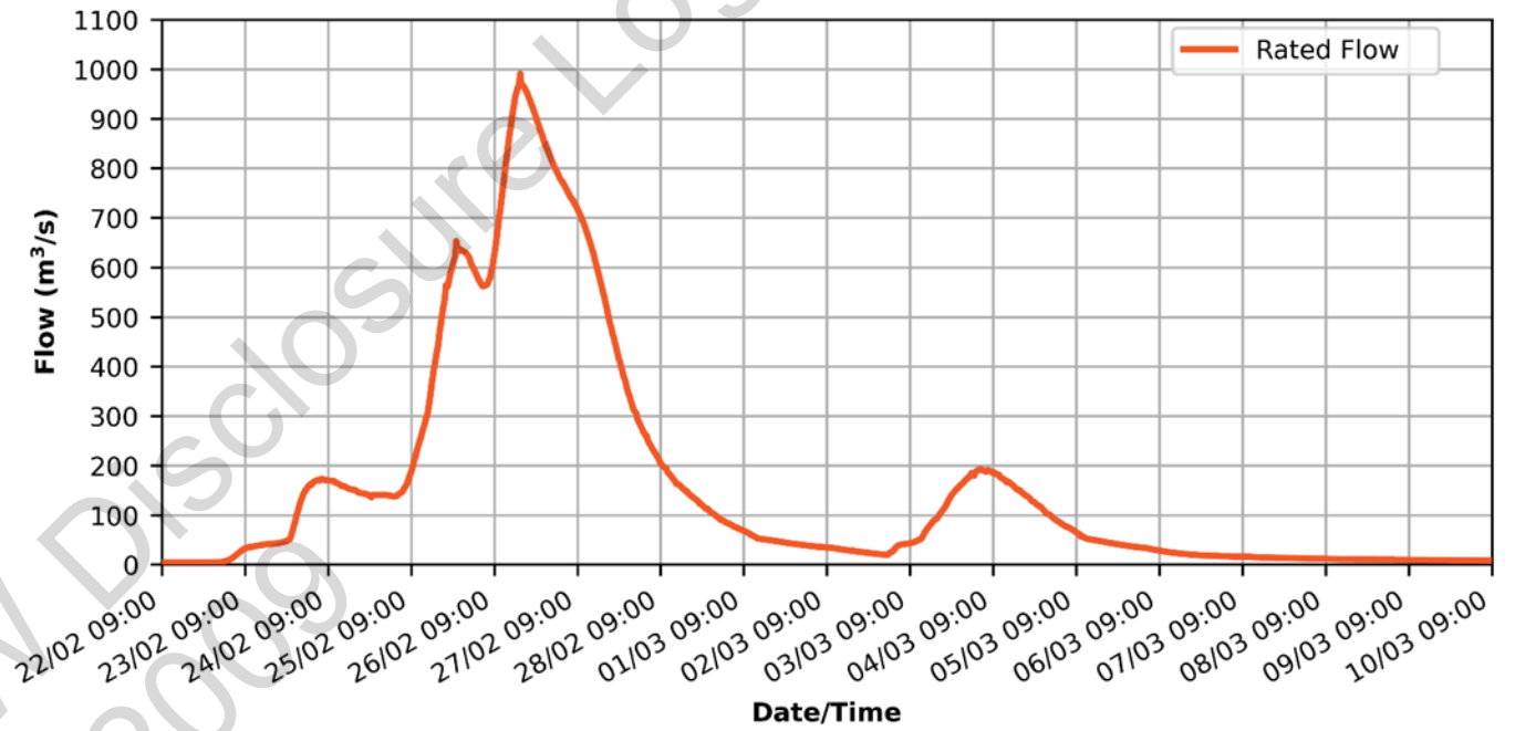
Figure 7-2: Rated flow for Stanley River at Woodford for the Flood Event
