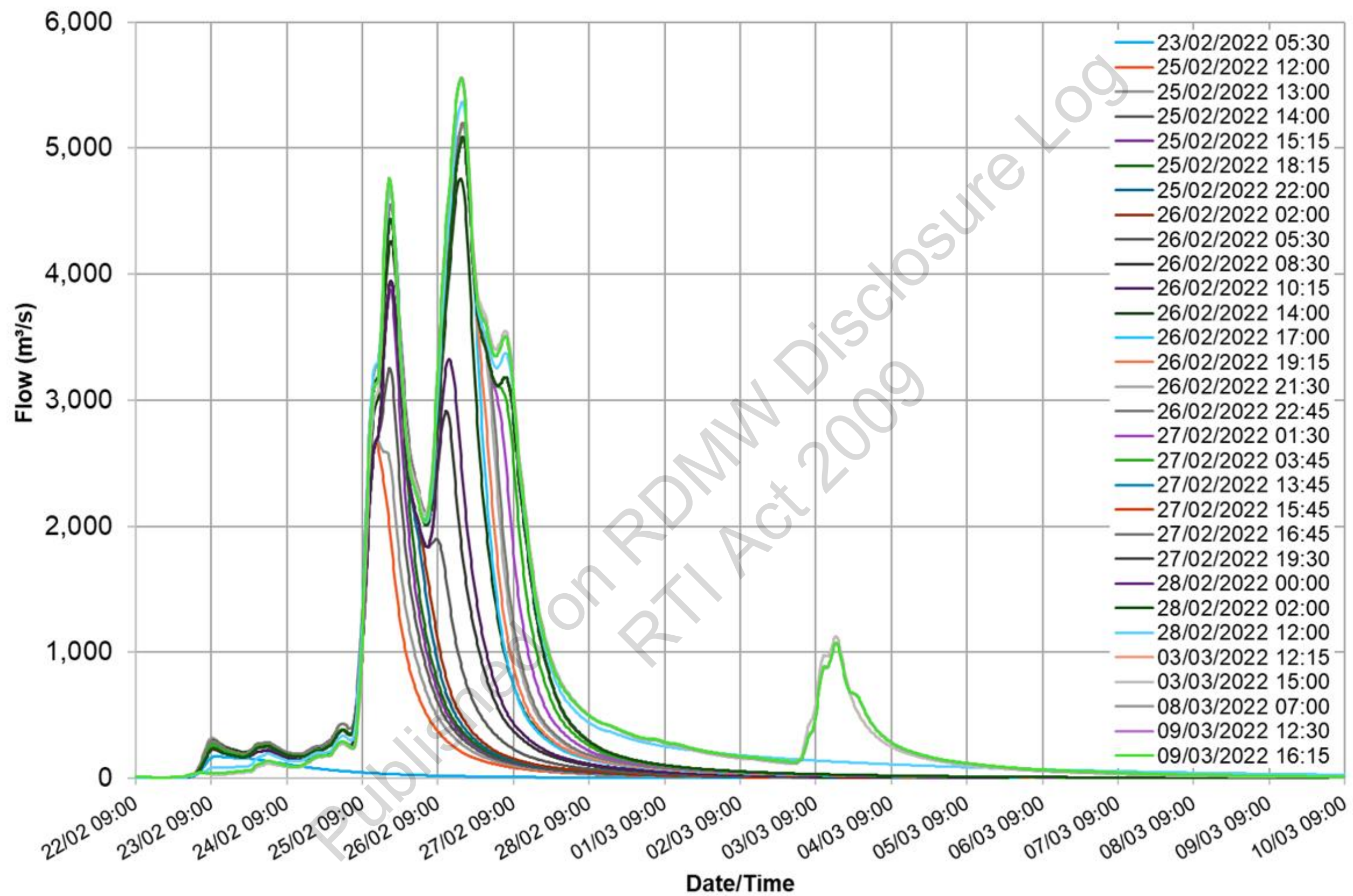
Figure 3-3: Modelled Somerset Dam inflow for each selected key model run
