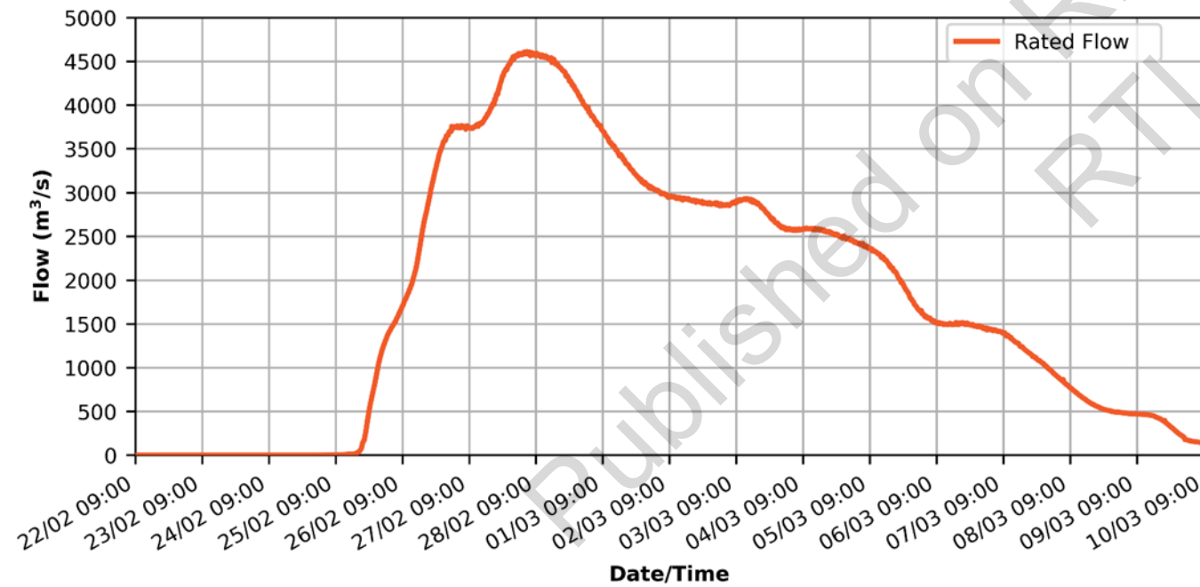
Figure 7-16: Rated flow for Brisbane River at Mt Crosby for the Flood Event
