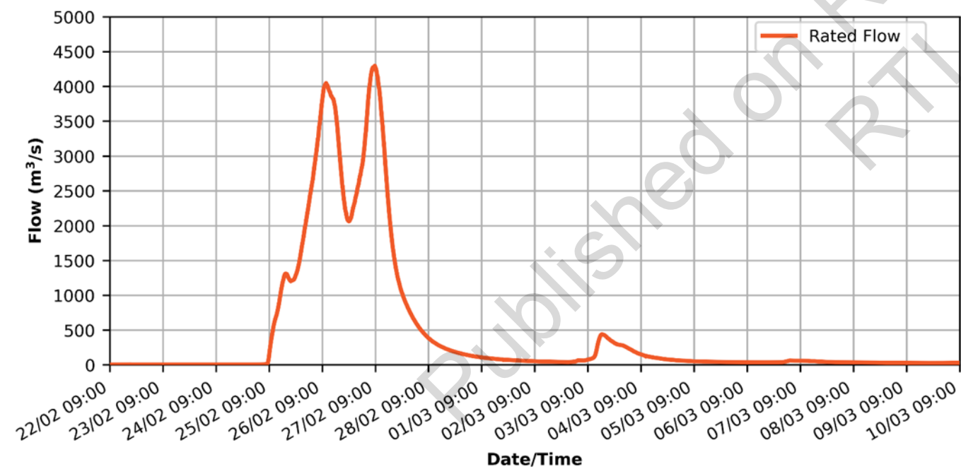
Figure 7-5: Rated flow for Brisbane River at Gregors Creek for the Flood Event
