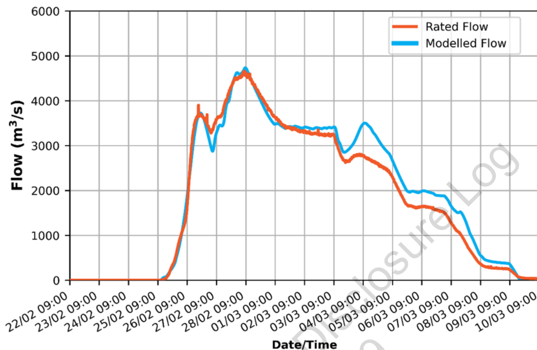
Figure 7-29: Whole of event calibration result (with the benefit of hindsight) at Lowood with revised Lockyer Creek parameter values to better match Lockyer Creek at Gatton
