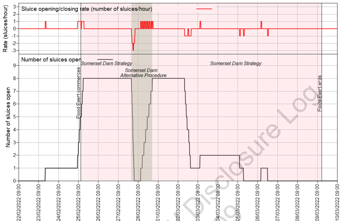
Figure 4-5: Somerset Dam total sluice opening and rate of change of sluice settings
