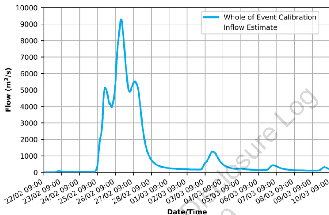
Figure 7-23: Wivenhoe Dam modelled inflow hydrograph excluding Somerset Dam releases produced by the post-event analysis whole of event calibration (with the benefit of hindsight)
