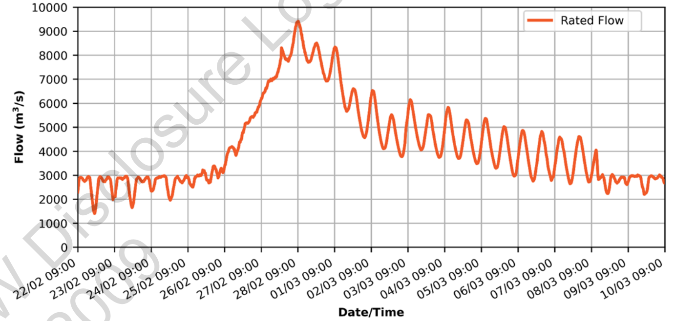
Figure 7-19: Rated flow for Brisbane River at Brisbane City for the Flood Event
