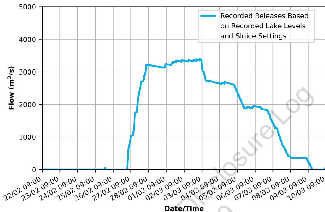
Figure 2-67: Wivenhoe Dam recorded release hydrograph for the period 22/02/2022 09:00 to 10/03/2022 09:00
