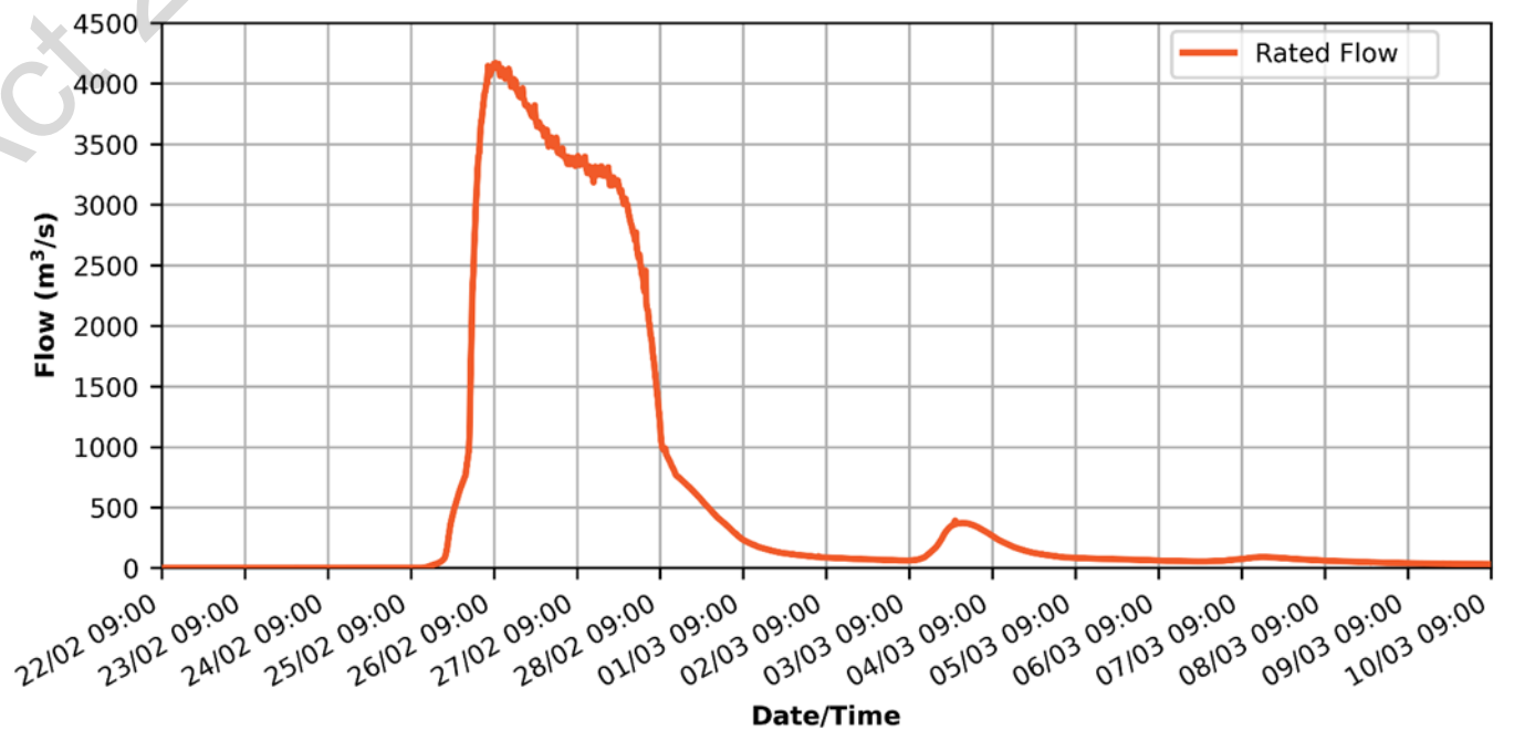
Figure 7-9: Rated flow for Lockyer Creek at Rifle Range Rd for the Flood Event
