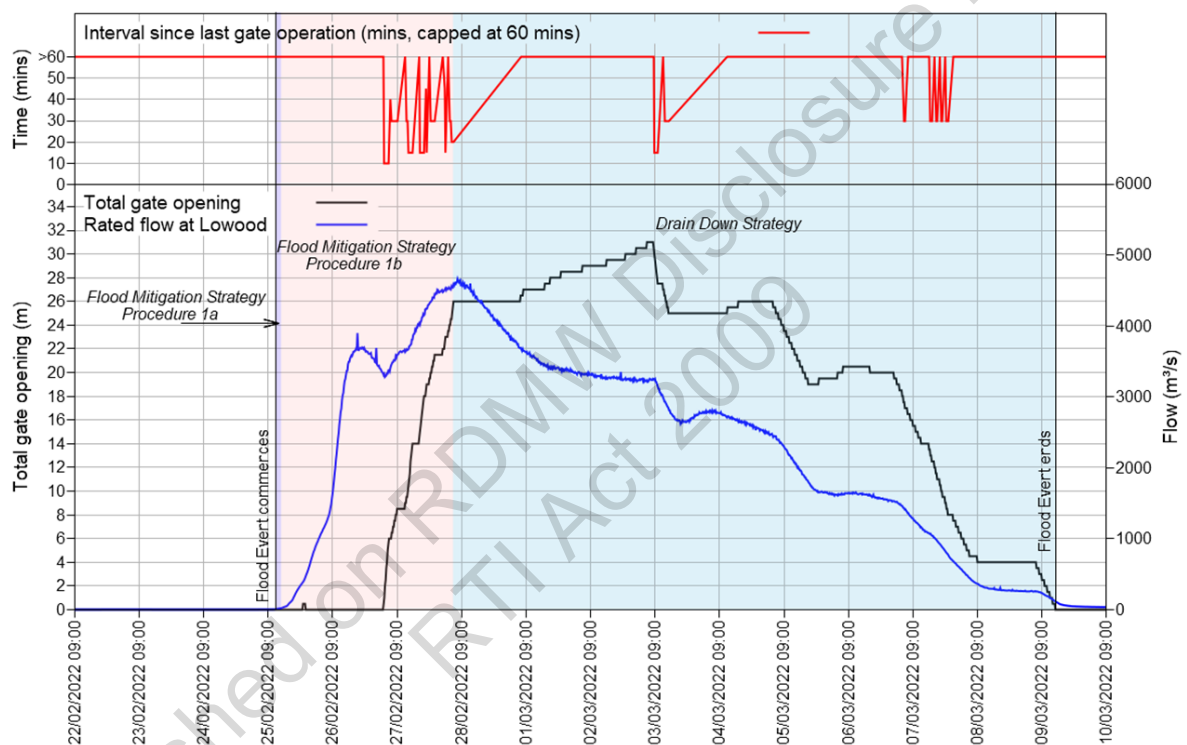
Figure 4-6: Wivenhoe Dam total gate opening, gate opening intervals and rated flow at Lowood
