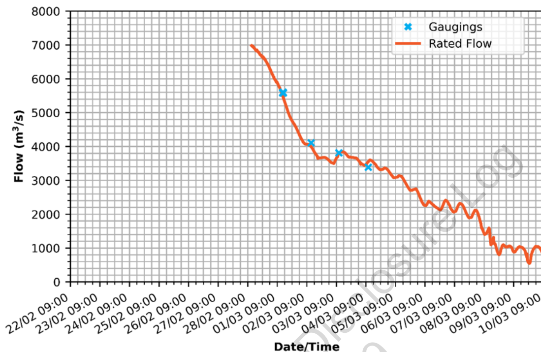
Figure 7-20: Comparison of gauged flow at Jindalee and rated flow
