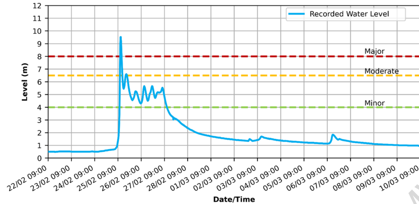
Figure 2-46: Recorded water level for Lockyer Creek at Helidon for the Flood Event
