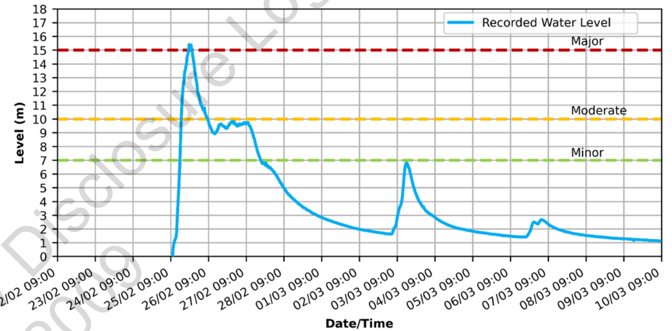
Figure 2-47: Recorded water level for Lockyer Creek at Gatton for the Flood Event
