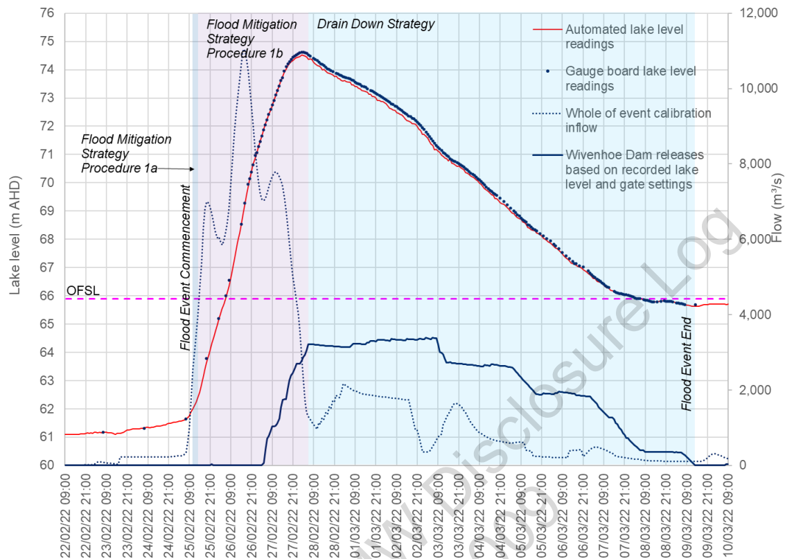
Figure ii: Wivenhoe Dam post-event analysis whole of event calibrated inflow, lake level (gauge board and automated readings) and releases (replicated in Figure 4-2)
