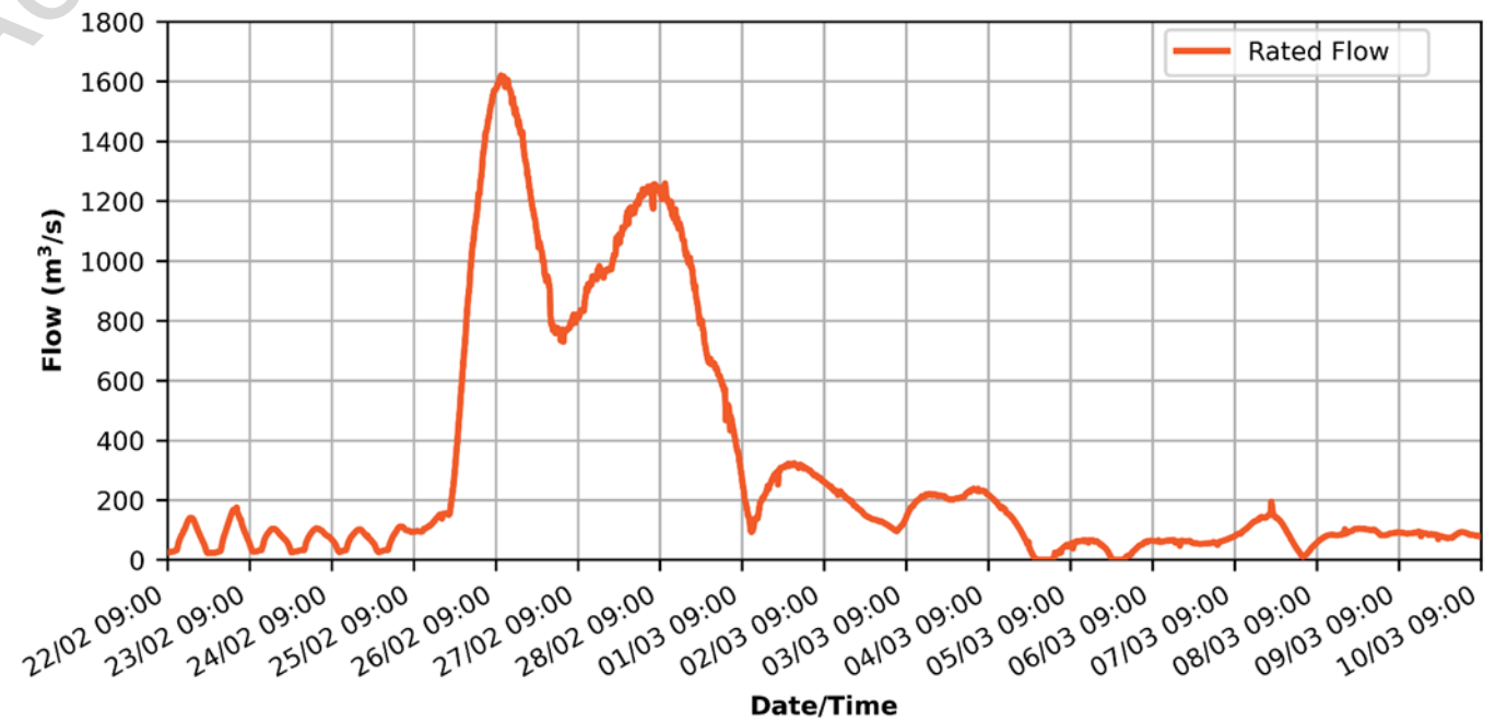
Figure 7-13: Rated flow for Bremer River at Ipswich for the Flood Event
