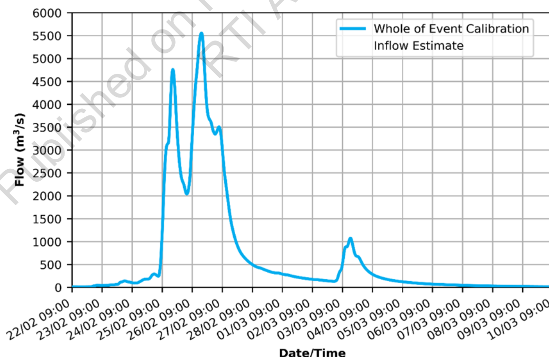
Figure 7-22: Somerset Dam modelled inflow hydrograph produced by the post-event analysis whole of event calibration (with the benefit of hindsight)
