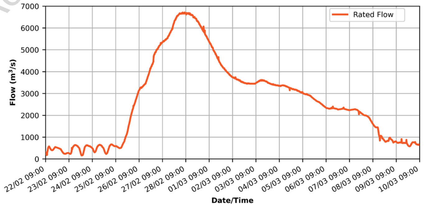
Figure 7-17: Rated flow for Brisbane River at Moggill for the Flood Event
