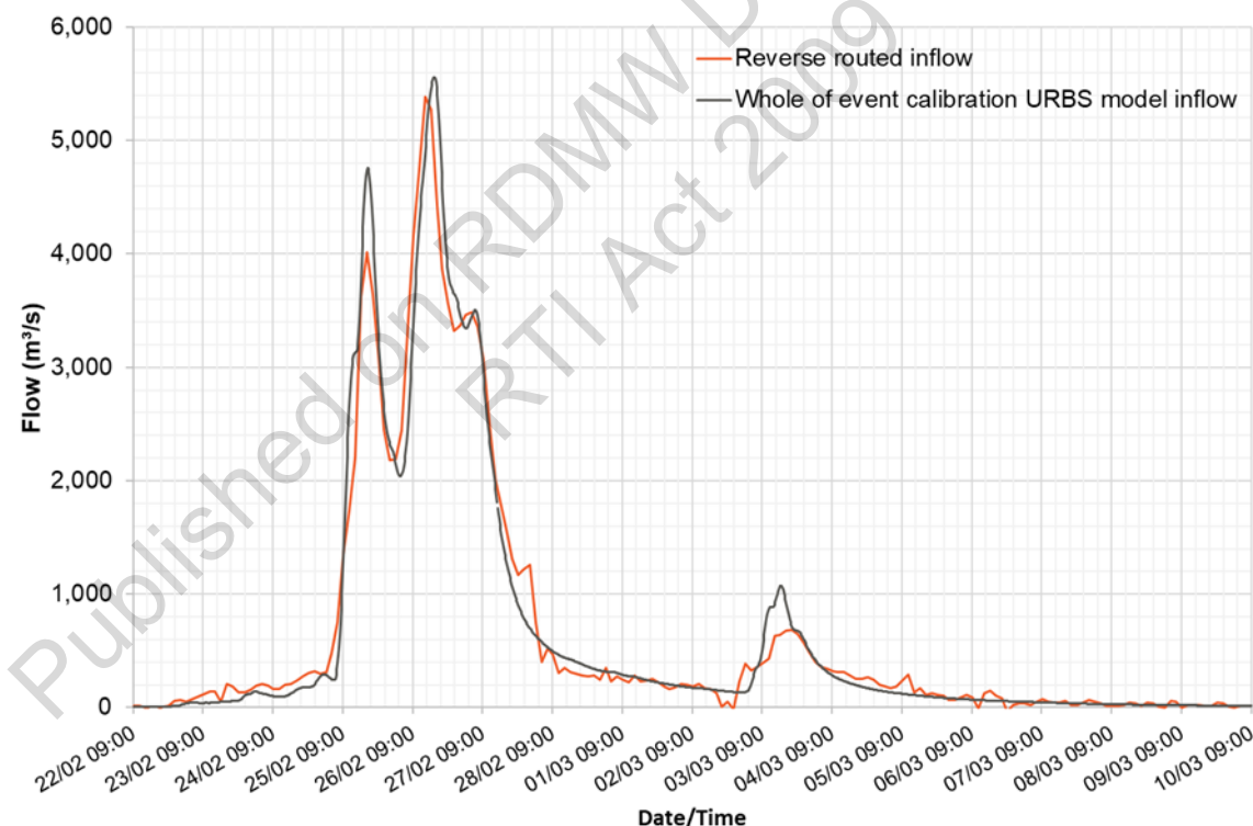
Figure 7-35: Post-event analysis reverse routed inflow calculation for Somerset Dam
