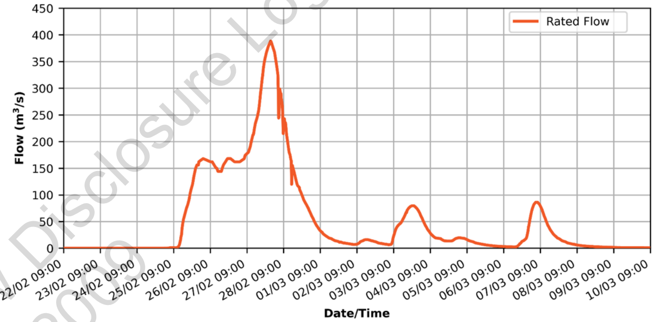
Figure 7-11: Rated flow for Purga Creek at Loamside for the Flood Event
