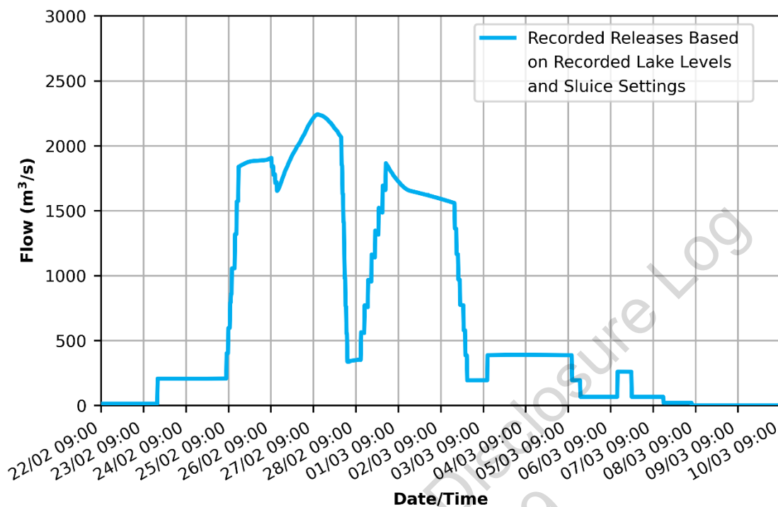
Figure 2-65: Somerset Dam recorded release hydrograph for the period 22/02/2022 09:00 to 10/03/2022 09:00
