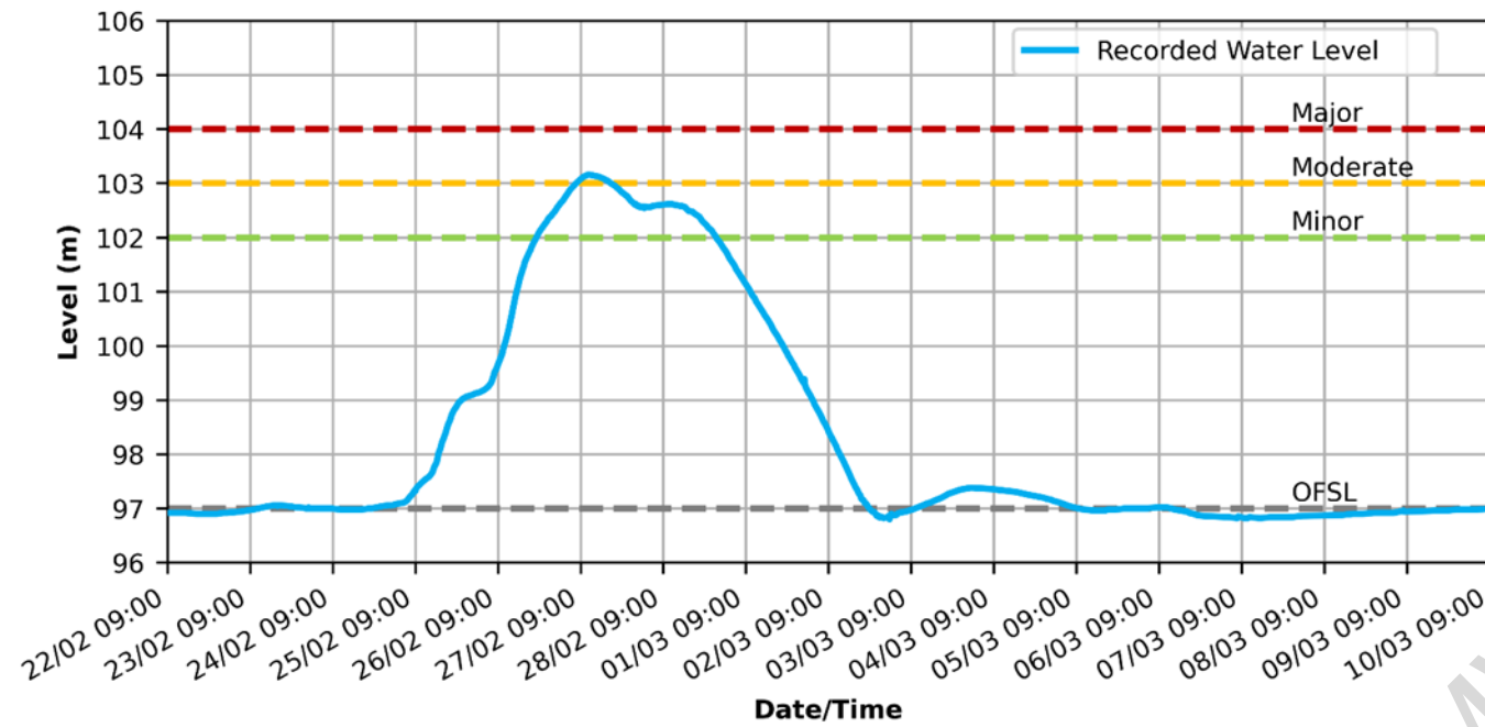
Figure 2-56: Recorded water level for Brisbane River at Lowood for the Flood Event
