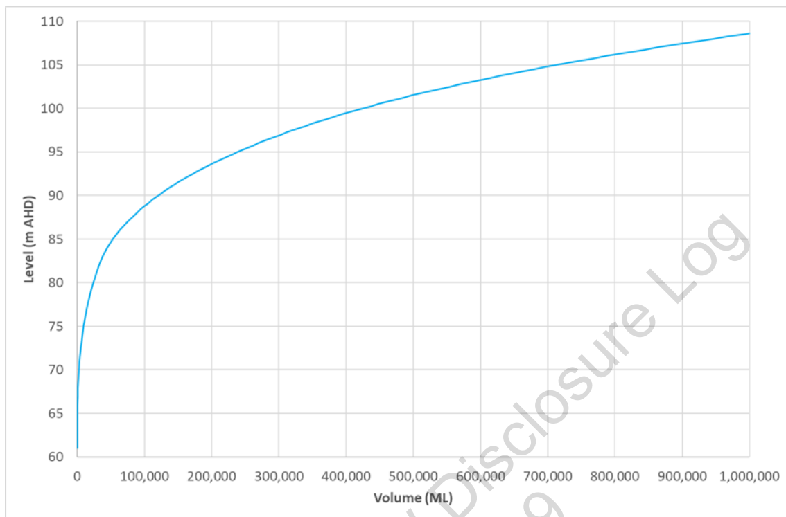
Figure 7-33: Somerset Dam storage-elevation relationship
