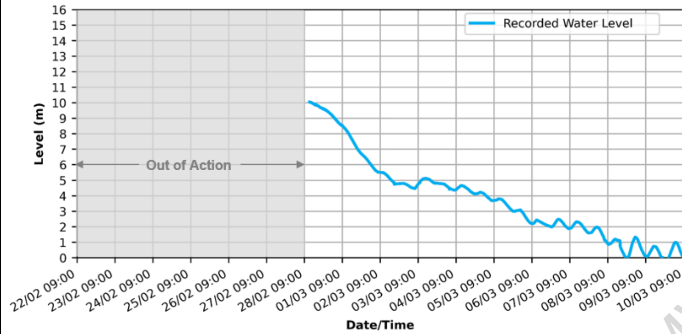
Figure 2-61: Recorded water level for Brisbane River at Jindalee for the Flood Event
