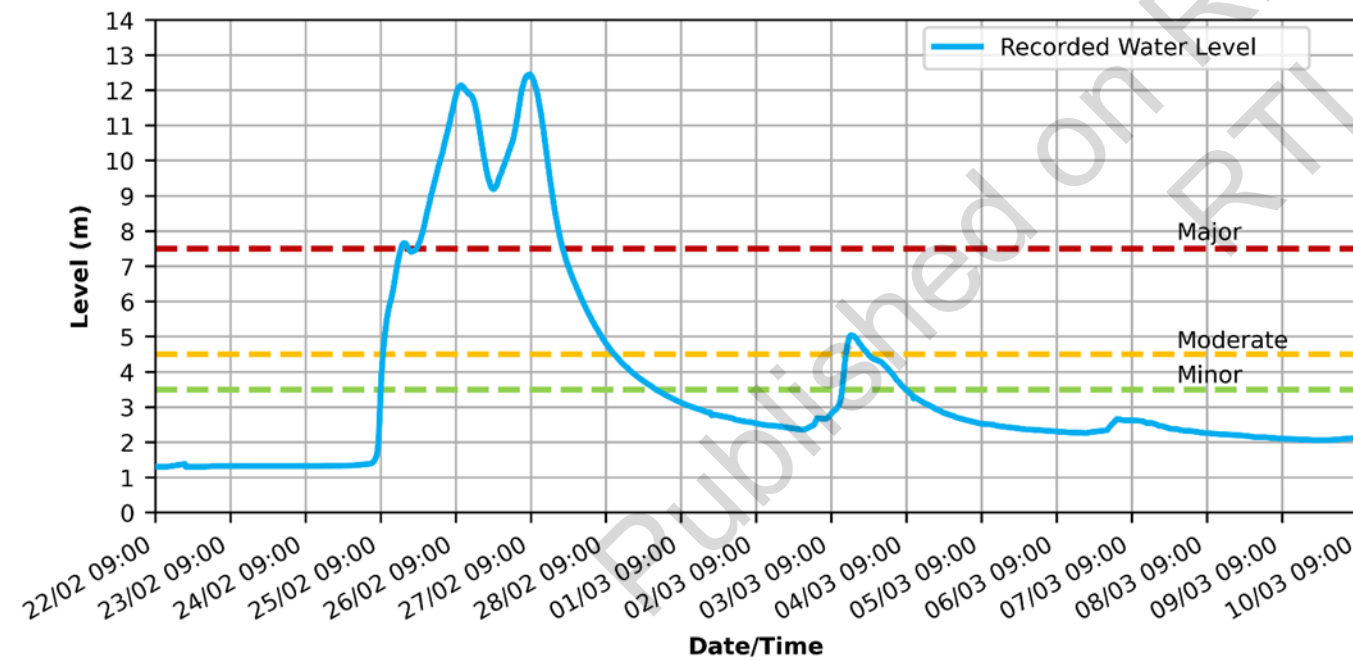
Figure 2-43: Recorded water level for Brisbane River at Gregors Creek for the Flood Event
