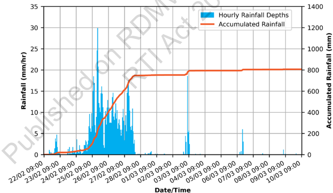
Figure 2-33: Bremer River catchment average rainfall in hourly increments and accumulated over the Flood Event for the period 22/02/2022 09:00 to 10/03/2022 09:00
