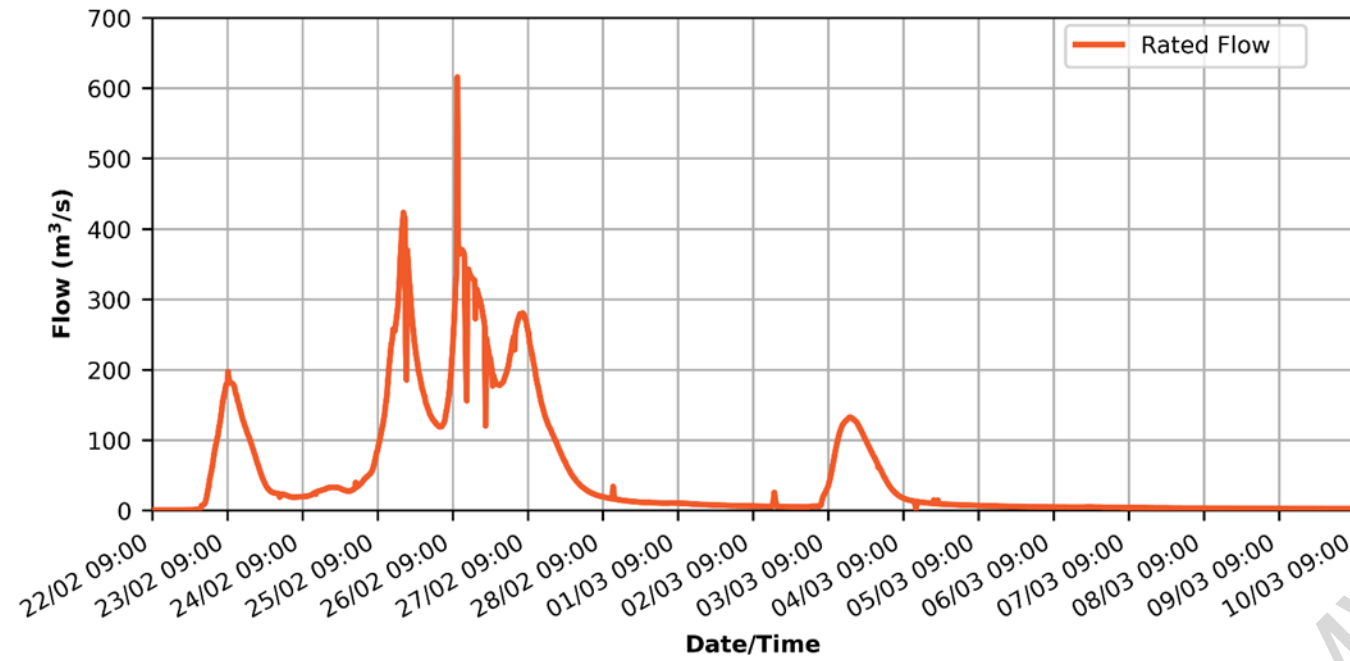
Figure 7-1: Rated flow for Stanley River at Peachester for the Flood Event
