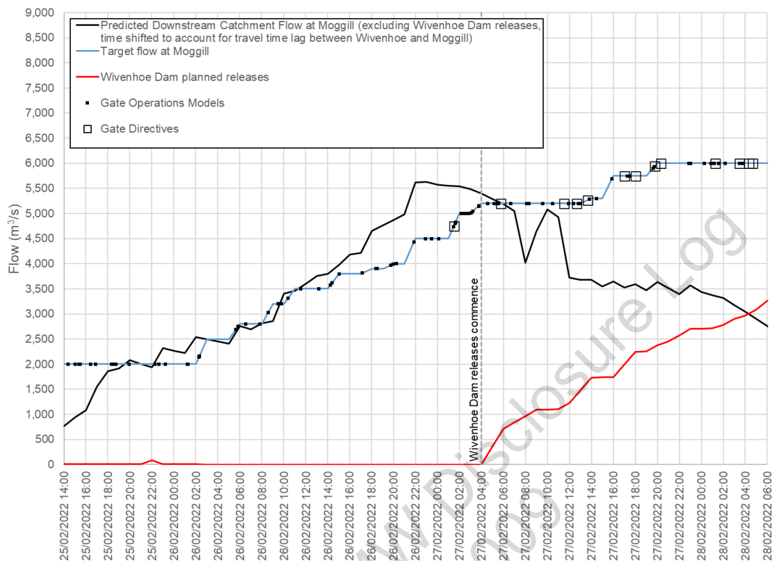
Figure 4-4: Wivenhoe Dam Flood Mitigation Strategy Procedure 1b release planning
