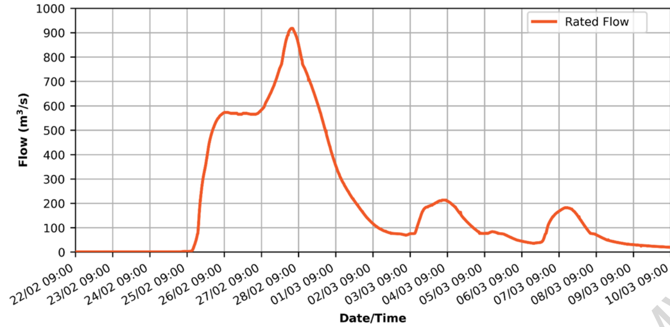
Figure 7-10: Rated flow for Warrill Creek at Amberley for the Flood Event
