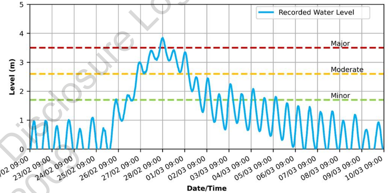
Figure 2-62: Recorded water level for Brisbane River at Brisbane City for the Flood Event
