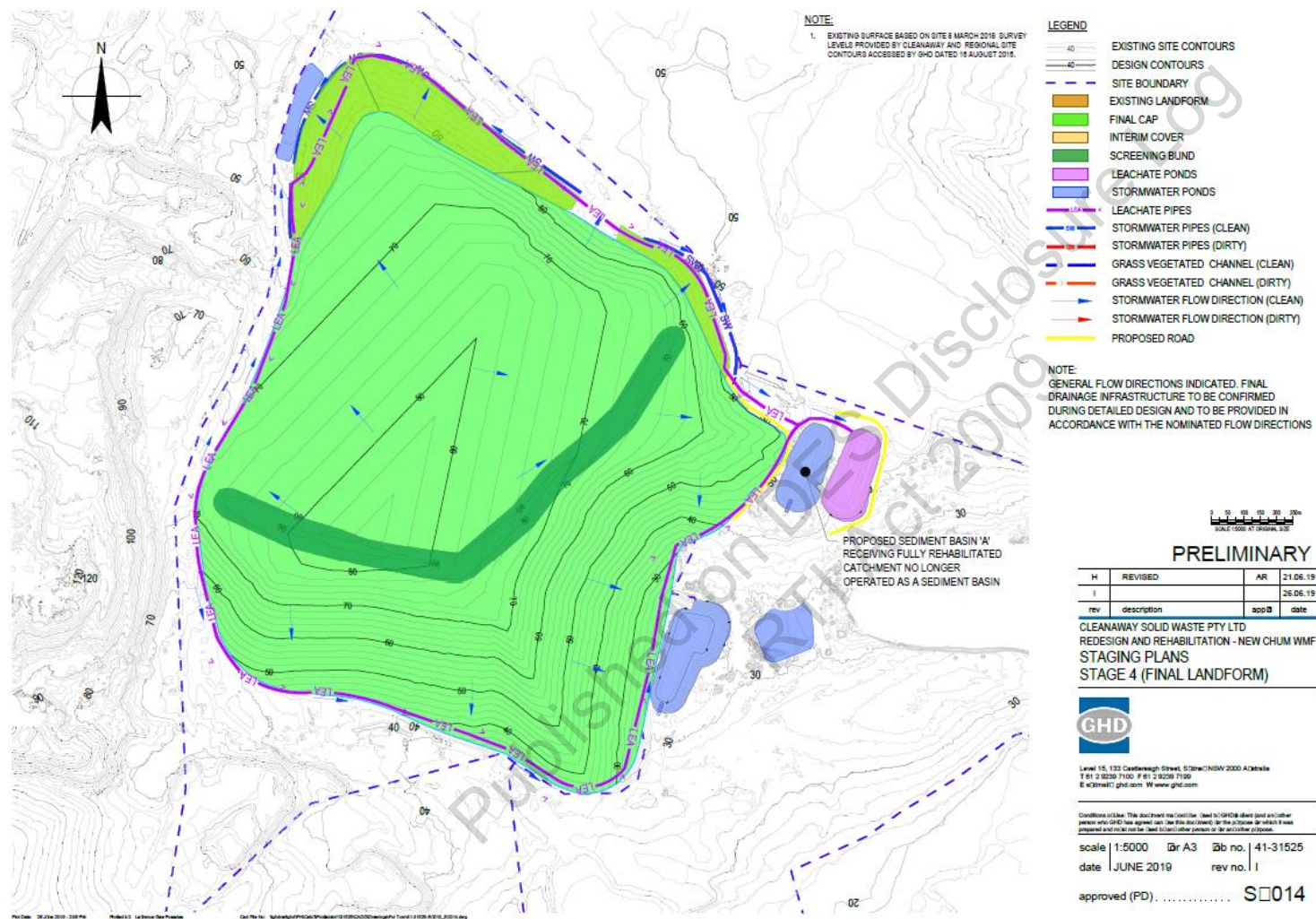
Figure 5: Lateral and vertical extension of the landfill (Stage 4 – final landform)
