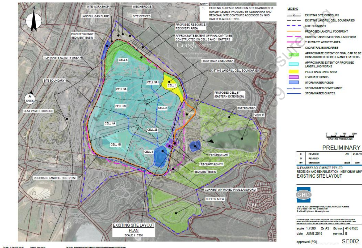
Figure 6: Existing landfill footprint
