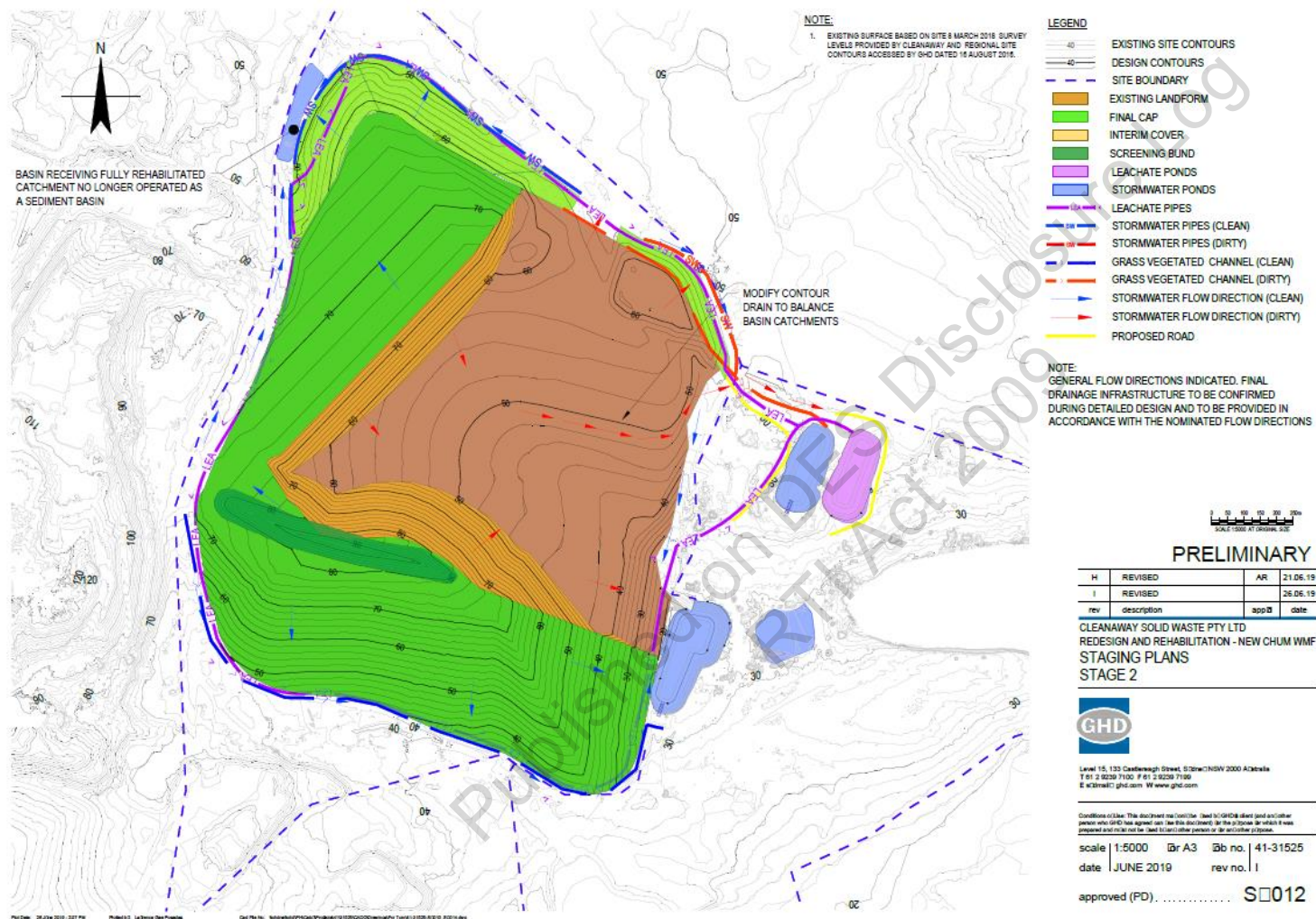
Figure 3: Lateral and vertical extension of the landfill (Stage 2)
