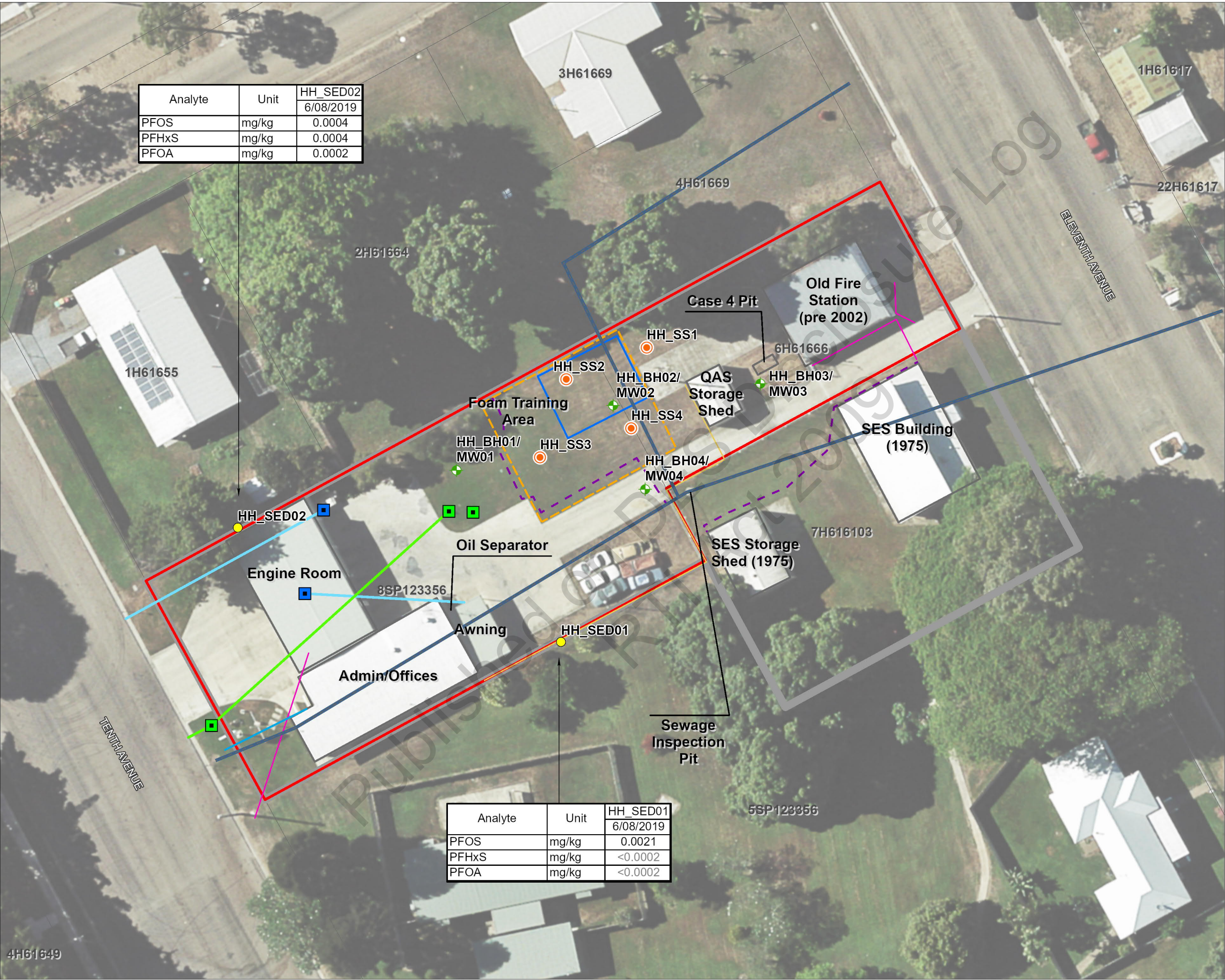
FIGURE 6 Sediment PFAS Analytical Results
