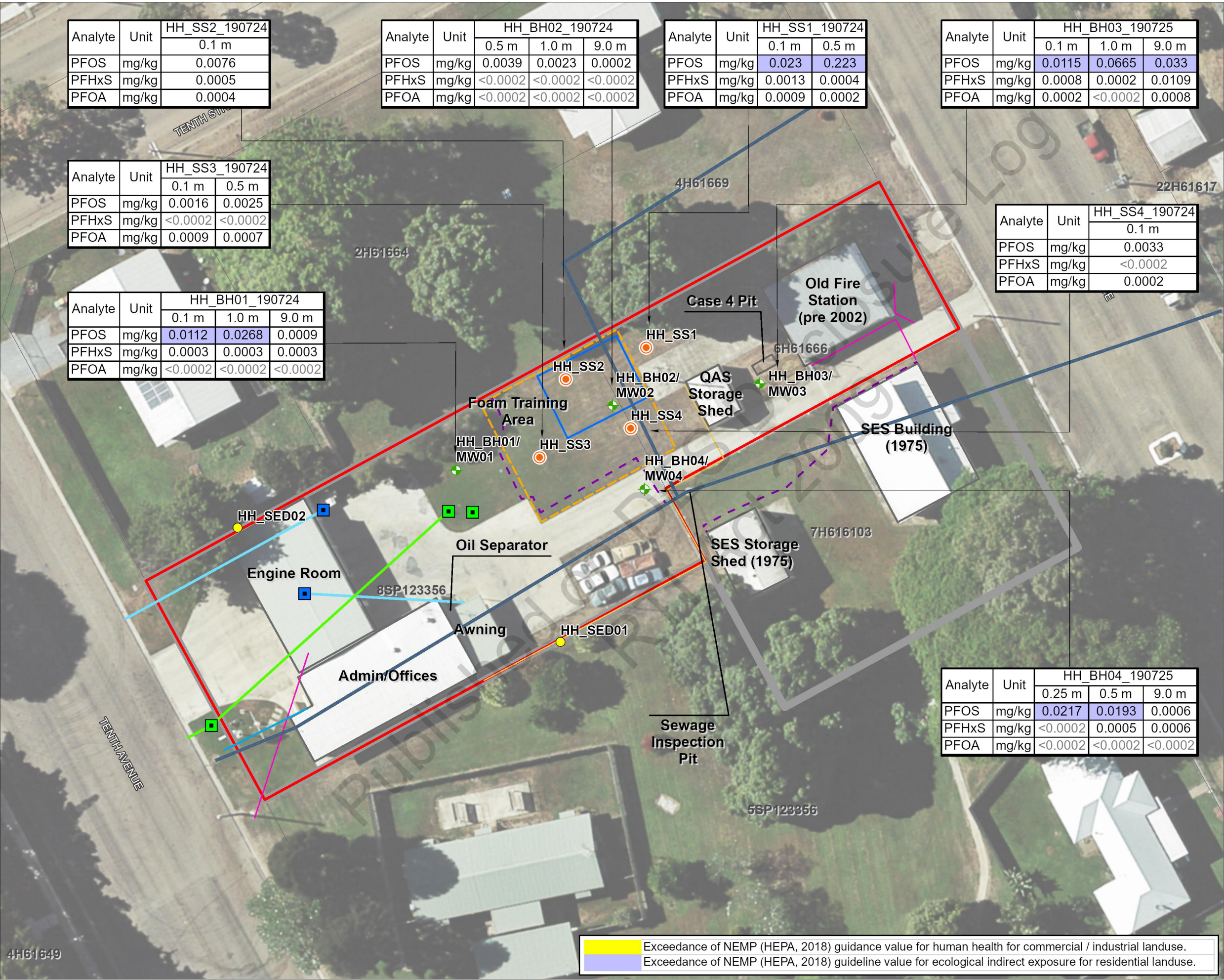
FIGURE 4 Soil PFAS Analytical Results
