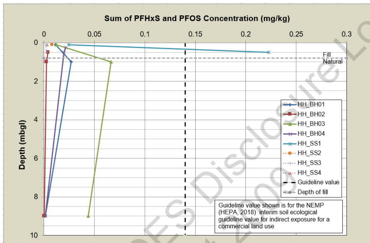
Chart 1 Concentration of \Sigma(\text{PFHxS}+\text{PFOS}) with depth in soil bores at Home Hill Fire Station
