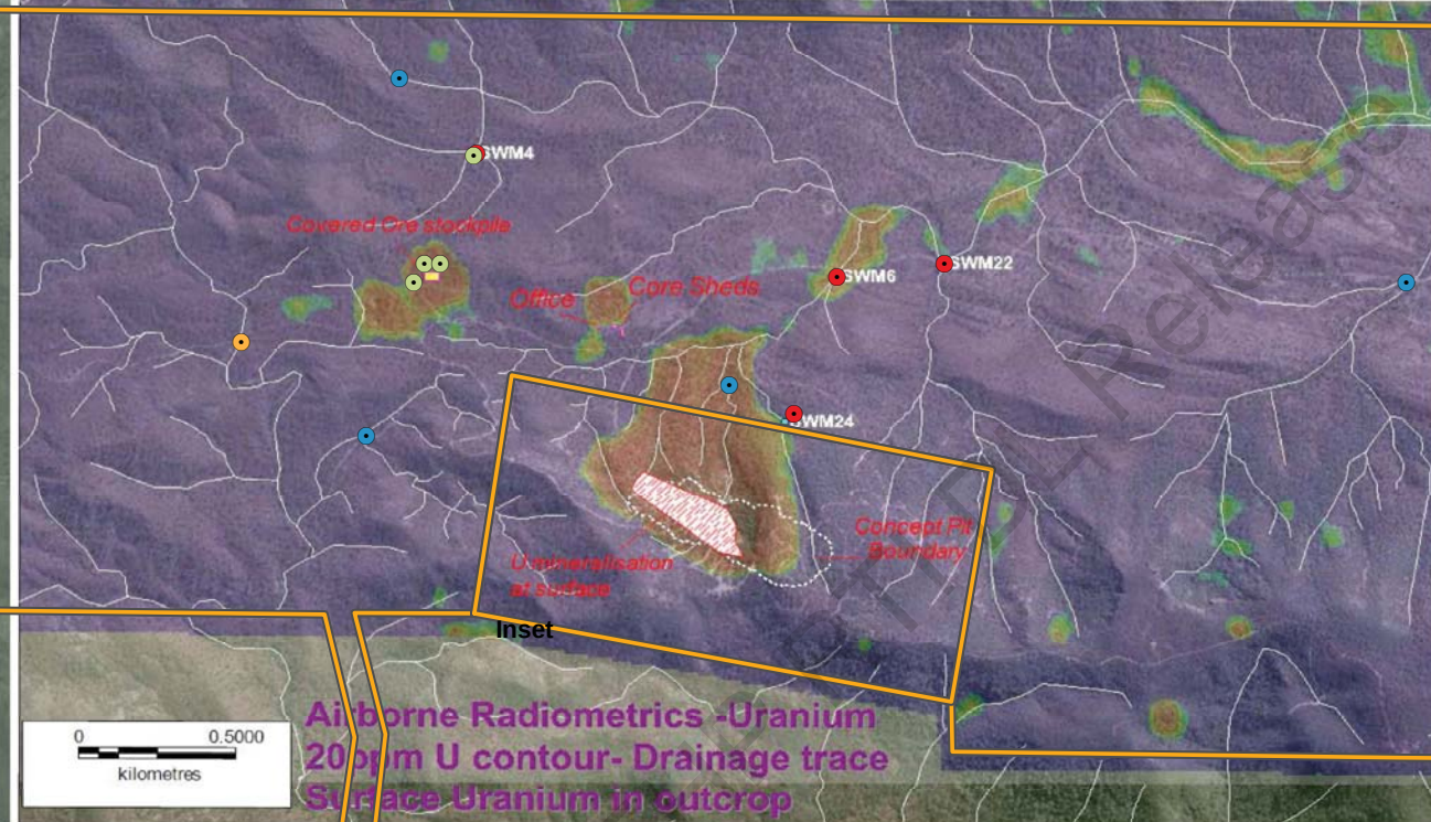
Figure 44 Airborne radiometrics locating surface uranium mineralisation in the Ben Lomond Mining Leases and SW sample provenance.
