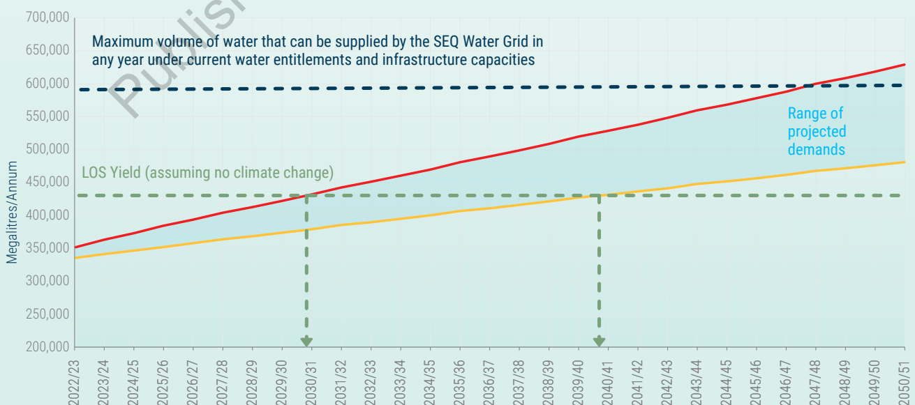
Figure 6 – Level of service yield of the existing system assuming no climate change
