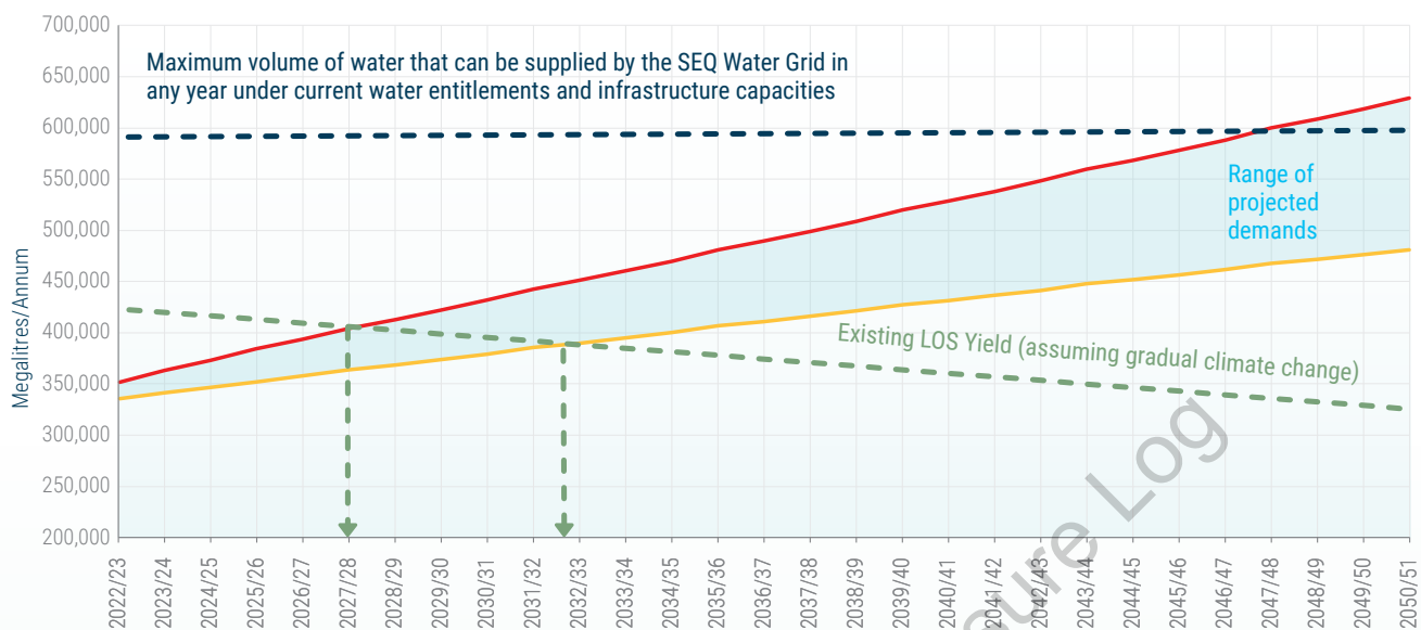
Figure 7 – Level of service yield of the existing system with gradual climate change prior to enhancement
