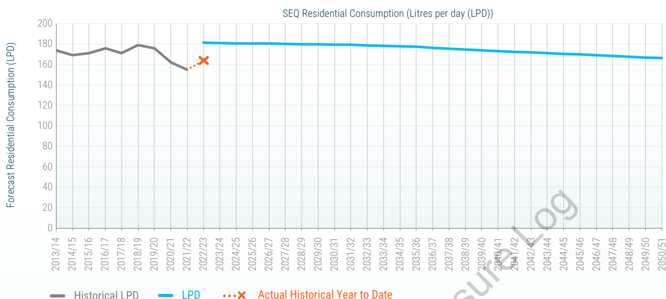
Figure 5 – Estimated projected regional average residential per capita urban water demands
