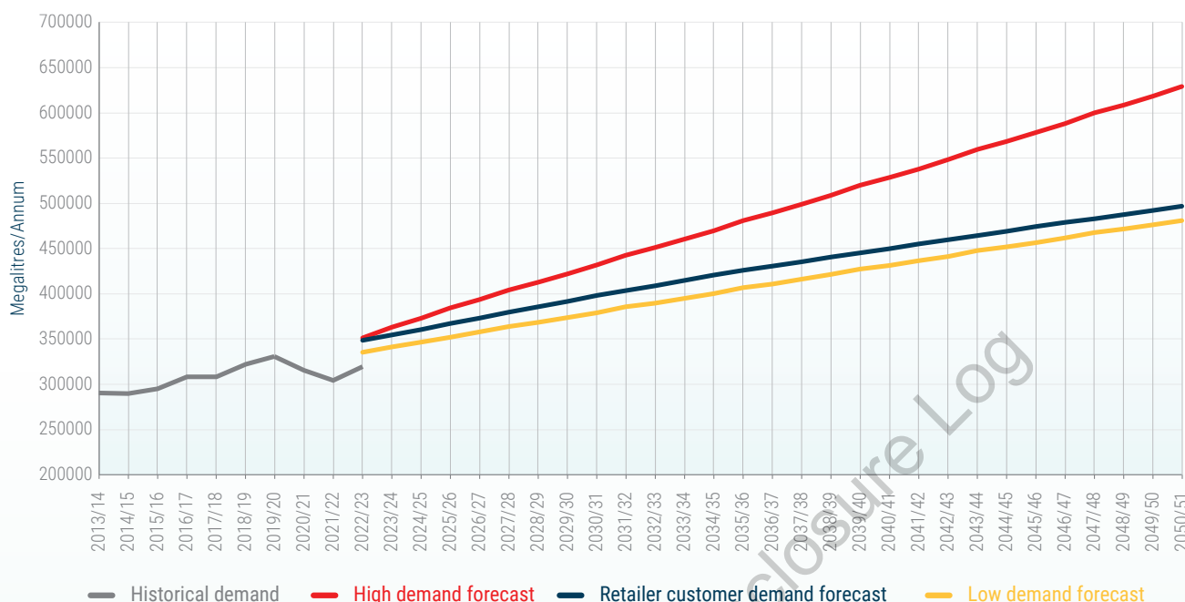
Figure 4 – Historical and projected South East Queensland water demands
