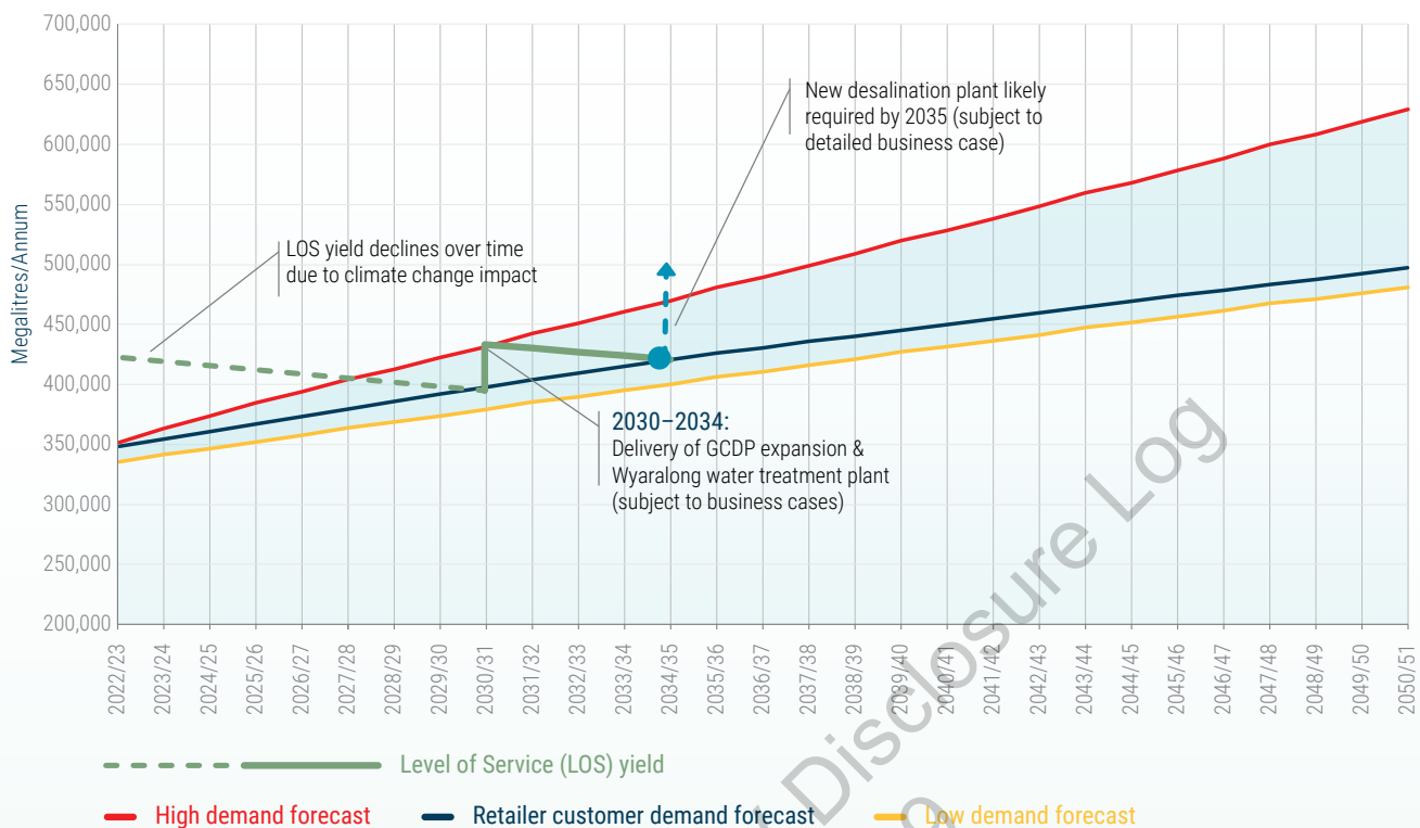
Figure 9 – Level of service yields including proposed future bulk water infrastructure upgrades
