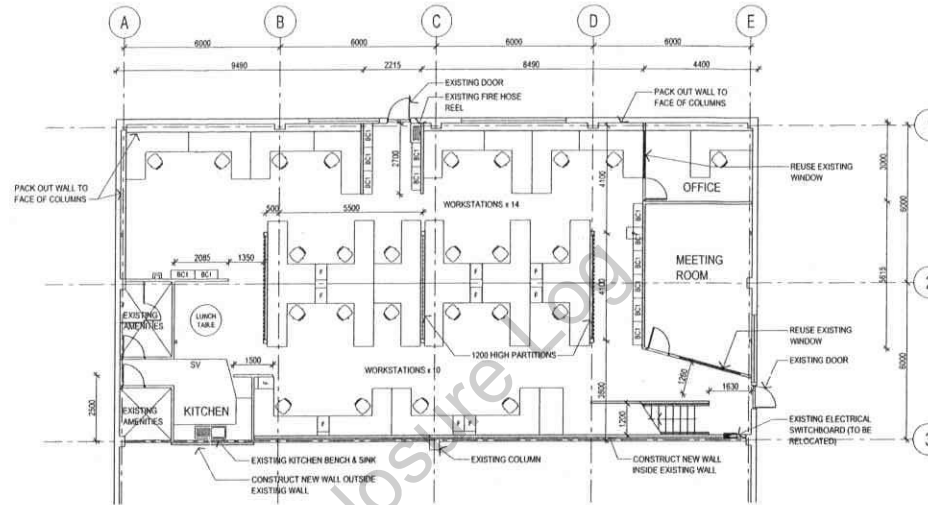
02 GROUND FLOOR PLAN SCALE 1:100
